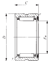
RNA49...U RNA69...U( F_w \leq 35 )
